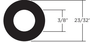
A402 (18.25mm O.D. x 9.52mm I.D.)
