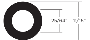
950573 (17.46mm O.D. x 9.92mm I.D.)
