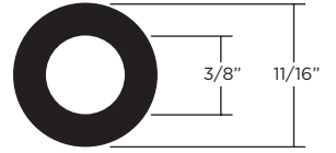
A403 (17.46mm O.D. x 9.52mm I.D.)
