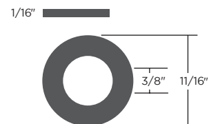
700767 (1.58mm x 9.52mm x 17.46mm)
