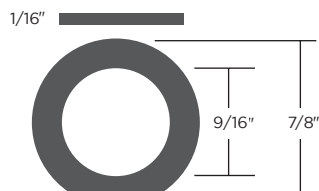
700769 (1.58mm x 14.28mm x 22.22mm)
