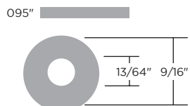
700780 (2.41mm x 5.15mm x 14.28mm)
