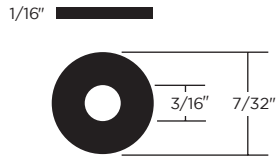
700603 A412 Size. Fits other makes. (1.59mm x 4.76mm x 5.55mm)
