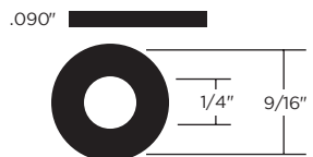
700737 Trumpet. (2.29mm x 6.35mm x 14.28mm)
