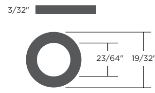
700771 (2.38mm x 9.12mm x 15.08mm)
