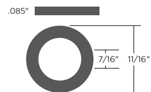
700775 (2.15mm x 11.11mm x 17.465mm)
