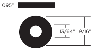
700691 Fits Eastman ETR-400 & similar. (2.41mm x 5.15mm x 14.58mm)
