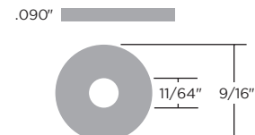
700762 (2.28mm x 4.36mm x 14.28mm)
