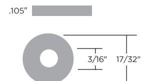
700778 (2.66mm x 4.76mm x 13.49mm)
