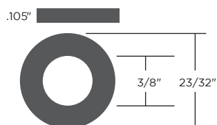
700773 (2.66mm x 9.52mm x 18.25mm)
