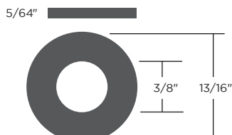
700770 (1.98mm x 9.52mm x 20.63mm)
