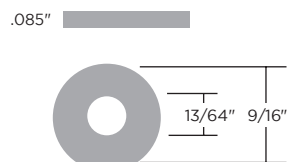
700777 (2.15mm x 5.15mm x 14.28mm)
