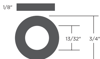
700768 (3.17mm x 10.31mm x 19.05mm)
