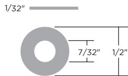
700756 (0.79mm x 5.55mm x 12.70mm)
